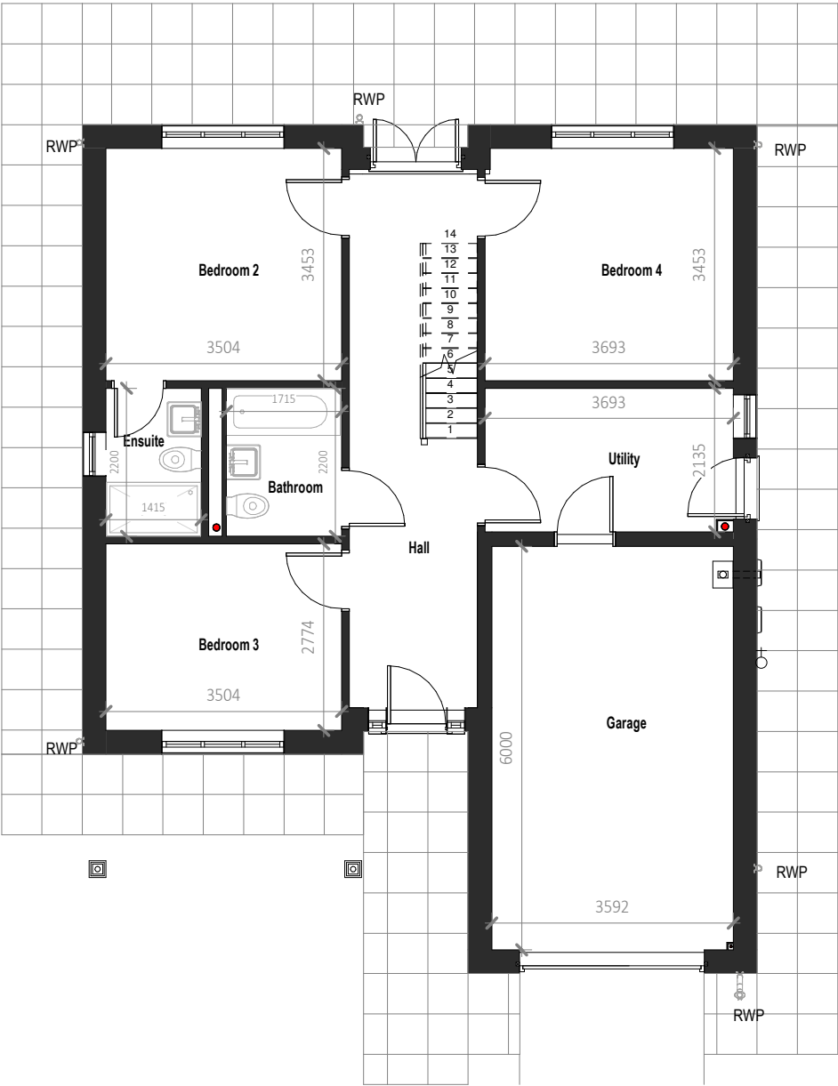
Ground Floor - Plan at A3 1 : 100 Plan at A1 1 : 50
